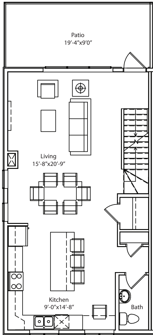
MAIN FLOOR 725 sq.ft
